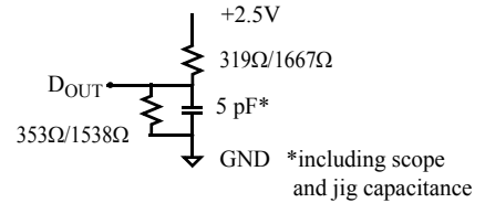
Figure C: Output load(B)
